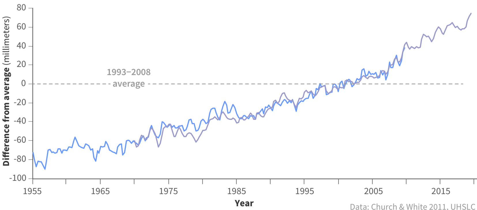
Global sea level (1955–2019)
